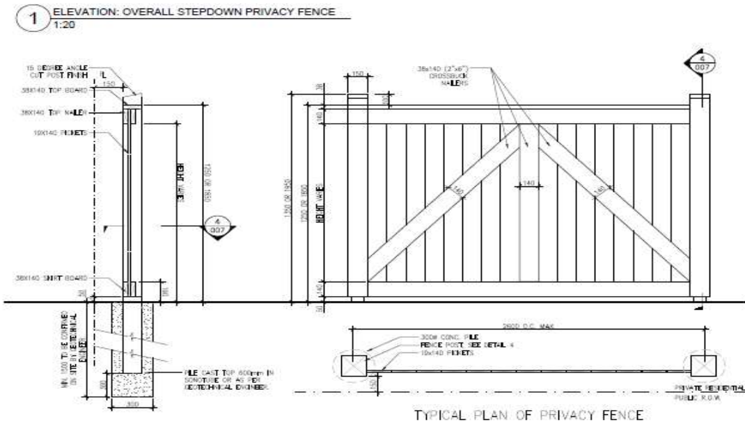
3 DETAIL: 1.2m HT. & 1.8m HT. PRIVACY FENCE SECTION & PANEL 1:20
